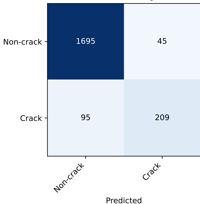
Predicted CE + robust aug.
