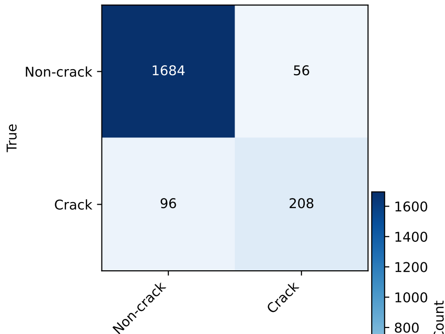
Predicted Focal + CBAM + robust\n( \gamma = 2 )
