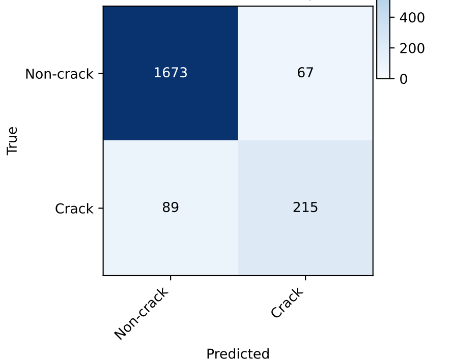
Predicted Focal + CBAM + robust\n( \gamma = 2 )
