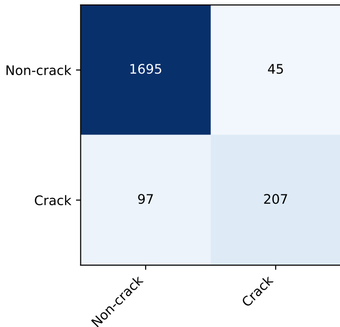
Predicted CE + robust aug.
