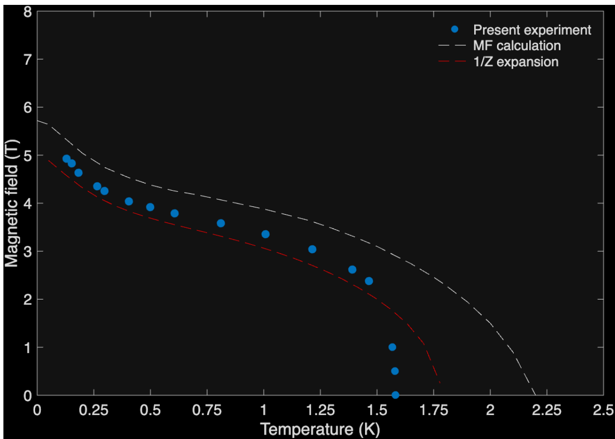
MF vs 1/z expansion
