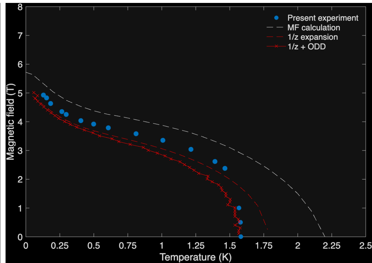
MF vs 1/z expansion vs 1/z + ODD
