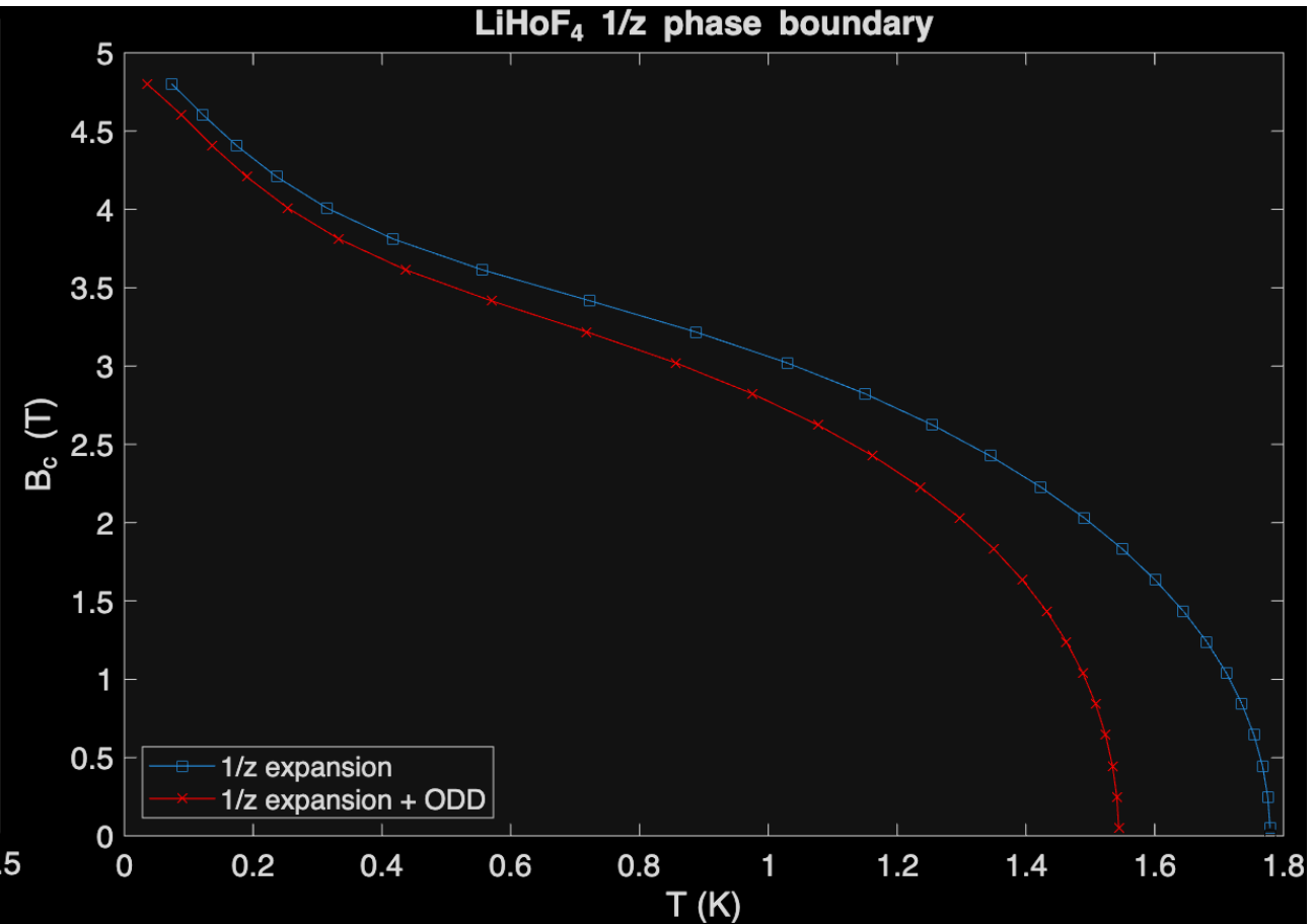
1/z expansion vs 1/z + \text{ODD}
