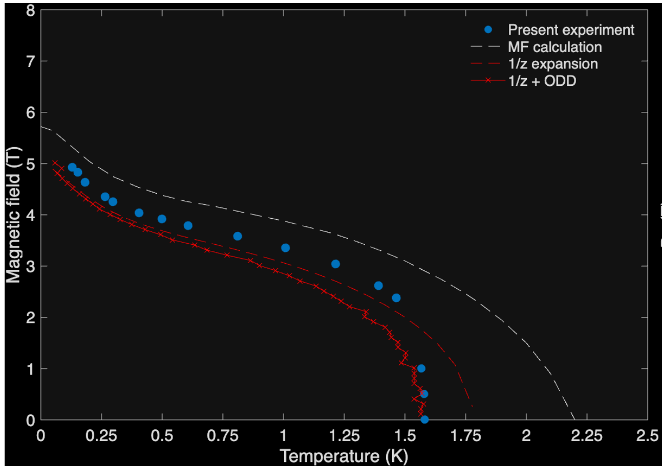
MF vs 1/z expansion vs 1/z + \text{ODD}
