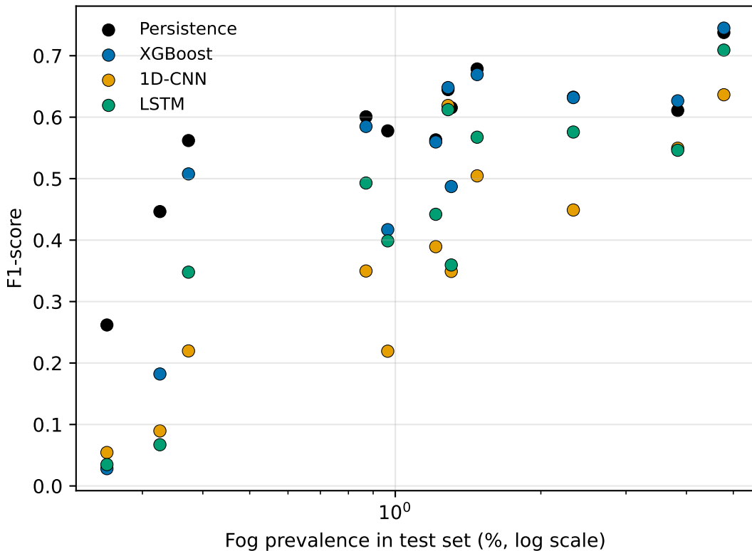
Overall T+1 performance vs. station fog prevalence
