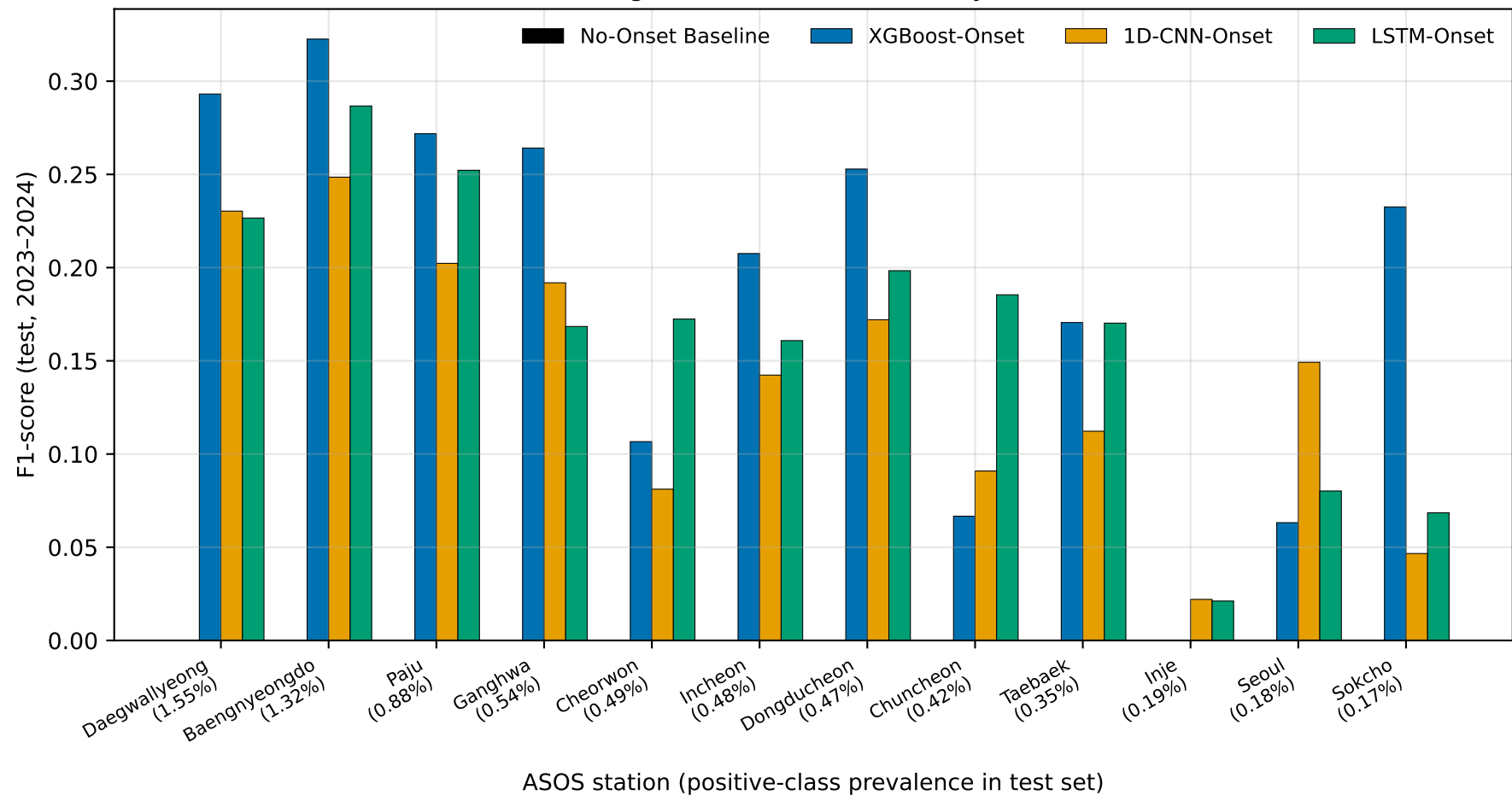
0→1 fog onset detection — F1 by station
