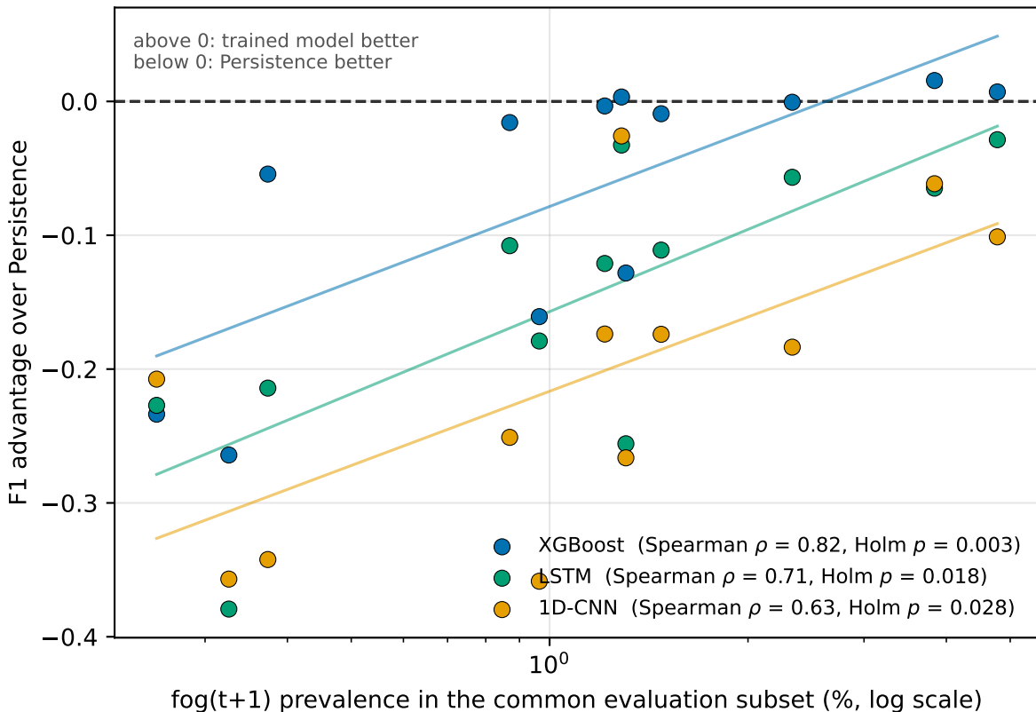
Trained-model advantage over Persistence vs. station fog prevalence
