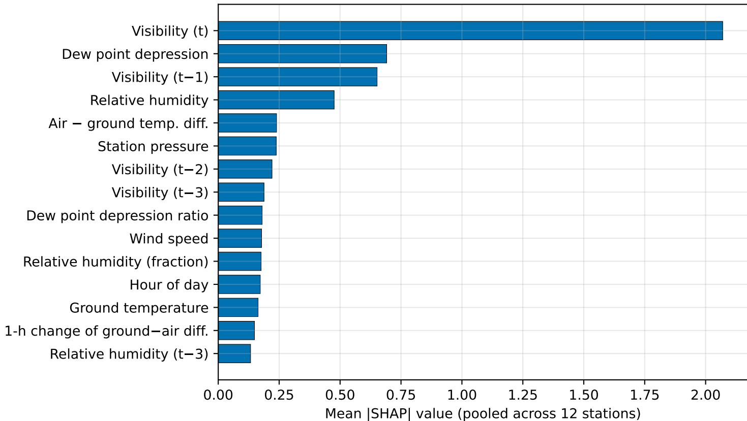
Global feature importance — overall T+1 XGBoost
