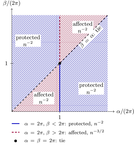
Figure 3: Gap-controlling parity and first correction scale in the bulk-critical limit. Region labels apply away from \alpha = 2\pi ; the colored segments give the separate boundary regime. Opposite hatching distinguishes the two parities in monochrome, and the solid/dashed boundary styles distinguish the two critical segments. The displayed window is schematic: all four regions continue throughout the positive (\alpha, \beta) quadrant.
