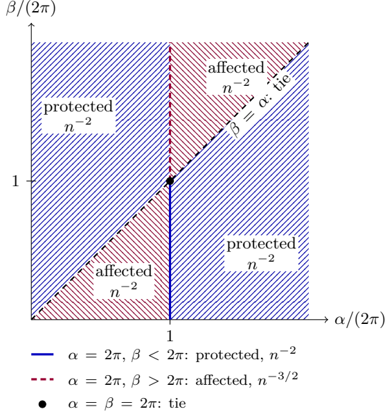
Figure 2: Gap-controlling parity and first correction scale in the bulk-critical limit. Region labels apply away from \alpha = 2\pi ; the colored segments give the separate boundary regime. Opposite hatching distinguishes the two parities in monochrome, and the solid/dashed boundary styles distinguish the two critical segments. The displayed window is schematic: all four regions continue throughout the positive (\alpha, \beta) quadrant.
