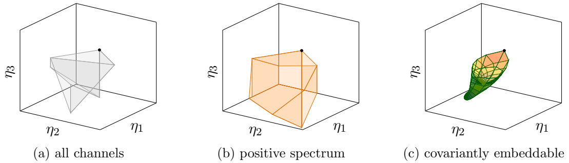
Figure 2: Spin 3/2. Panels (a) and (b) are generated from exact rational polytope vertices. Panel (c) renders the three boundary surfaces obtained by setting one canonical rate to zero; each displayed surface uses rates in [0, 8] , while the defining cone is unbounded.
