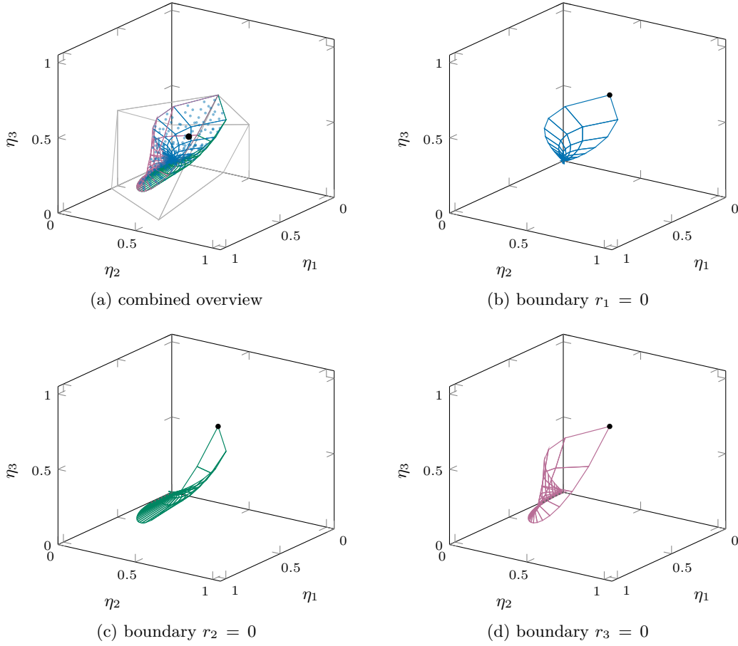
Figure 3. Spin 3/2 embeddable geometry, with identical axes and viewing angles in all panels. Panel (a) shows the three boundary meshes and sampled embeddable interior inside the faint nonnegative-spectrum polytope; the black point is e^{-1}(1, 1, 1) . Panels (b)–(d) separate the surfaces by the canonical rate set to zero, with the identity marked. The exact region is defined by inequalities (5.14)–(5.16). Each mesh samples the two free integrated rates over [0, 8] . Gray dotted edges in panels (b)–(d) mark rendering cutoffs, not additional mathematical boundaries. Interior dots are samples, not a description of the full region.
