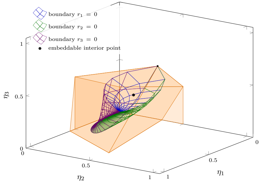
Figure 3. Spin 3/2 embeddable geometry. The three colored boundary meshes are overlaid on the orange nonnegative-spectrum polytope and are labeled by the canonical rate set to zero. The embeddable region is the common side of the sheets containing the marked diagonal point e^{-1}(1, 1, 1) . The two free rates on each mesh range over [0, 8] , while the defining cone is unbounded. The heavier dashed mesh edges are sampling cutoffs, not mathematical boundary curves.
