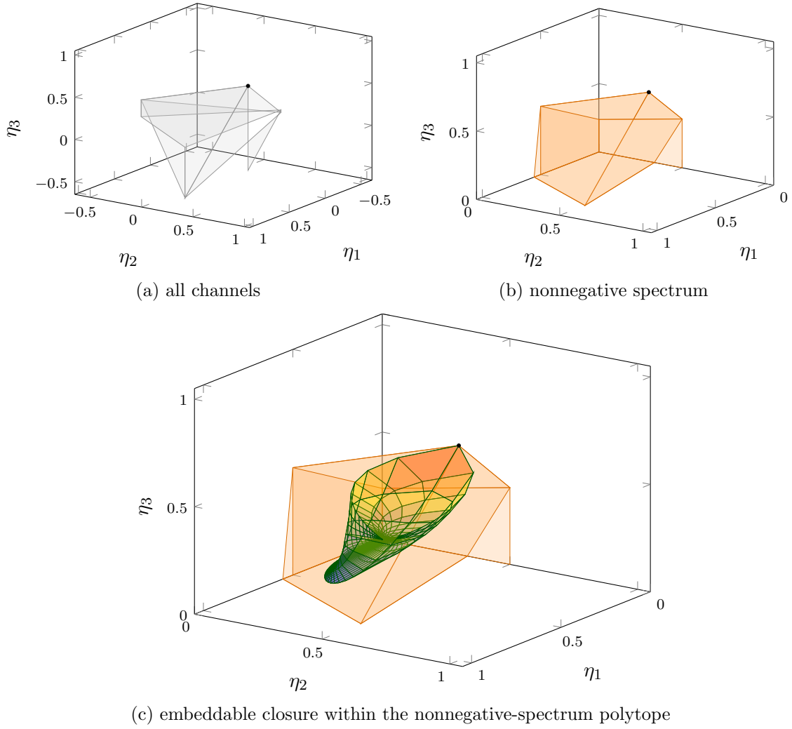
Figure 2: Spin 3/2. Panels (a) and (b) are generated from exact rational polytope vertices. Panel (c) overlays the three green embeddable-boundary surfaces on the orange nonnegative-spectrum polytope. Each surface is obtained by setting one canonical rate to zero and uses the other rates in [0, 8] , while the defining cone is unbounded.
