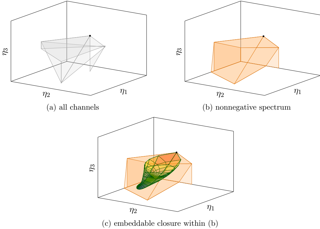
Figure 2: Spin 3/2. Panels (a) and (b) are generated from exact rational polytope vertices. Panel (c) overlays the three green embeddable-boundary surfaces on the orange nonnegative-spectrum polytope. Each surface is obtained by setting one canonical rate to zero and uses the other rates in [0, 8] , while the defining cone is unbounded.
