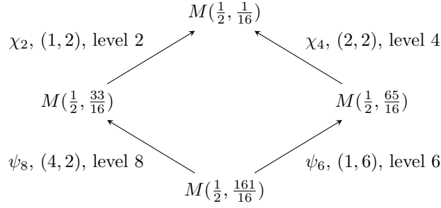
Figure 2: The spin diamond. The two branches meet first at total level 10, where \chi_{10} = j_{\chi_2}(\psi_8) = j_{\chi_4}(\psi_6) creates the double pole of Theorem 9.4.
