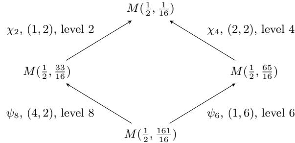
Figure 2. The spin diamond. The two branches meet first at total level 10, where \chi_{10} = j_{\chi_2}(\psi_8) = j_{\chi_4}(\psi_6) creates the double pole of Theorem 9.5.
