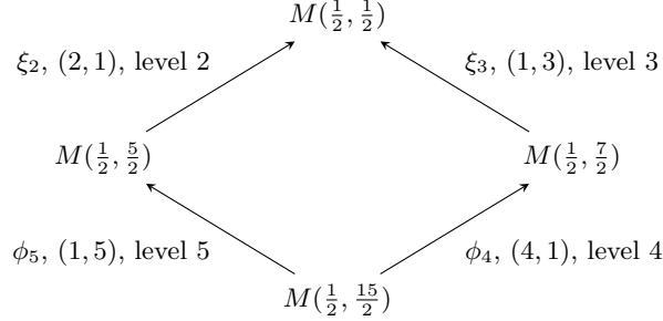
Figure 1. The energy diamond. Arrows are the singular-vector embeddings of Proposition 8.1, labelled by the embedded singular vector, its Kac label, and its relative level. The two branches meet first at total level 7, where \xi_7 = j_{\xi_2}(\phi_5) = j_{\xi_3}(\phi_4) creates the first double pole of the Ising block.
