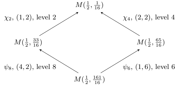
Figure 2. The spin diamond. The two branches meet first at total level 10, where \chi_{10} = j_{\chi_2}(\psi_8) = j_{\chi_4}(\psi_6) creates the double pole of Theorem 9.5.
