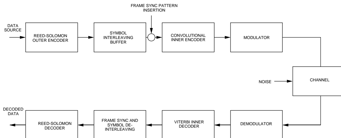
Figure 6-1: Concatenated Coding System Block Diagram
