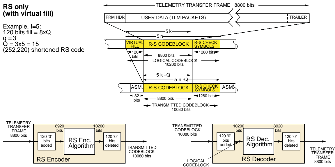
Figure 5-3: Illustration of RS Codeword Structure, with and without Virtual Fill
