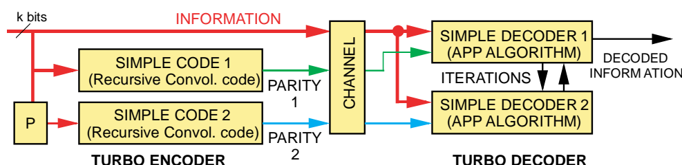
Figure 7-1: Example of Turbo Encoder/Decoder
