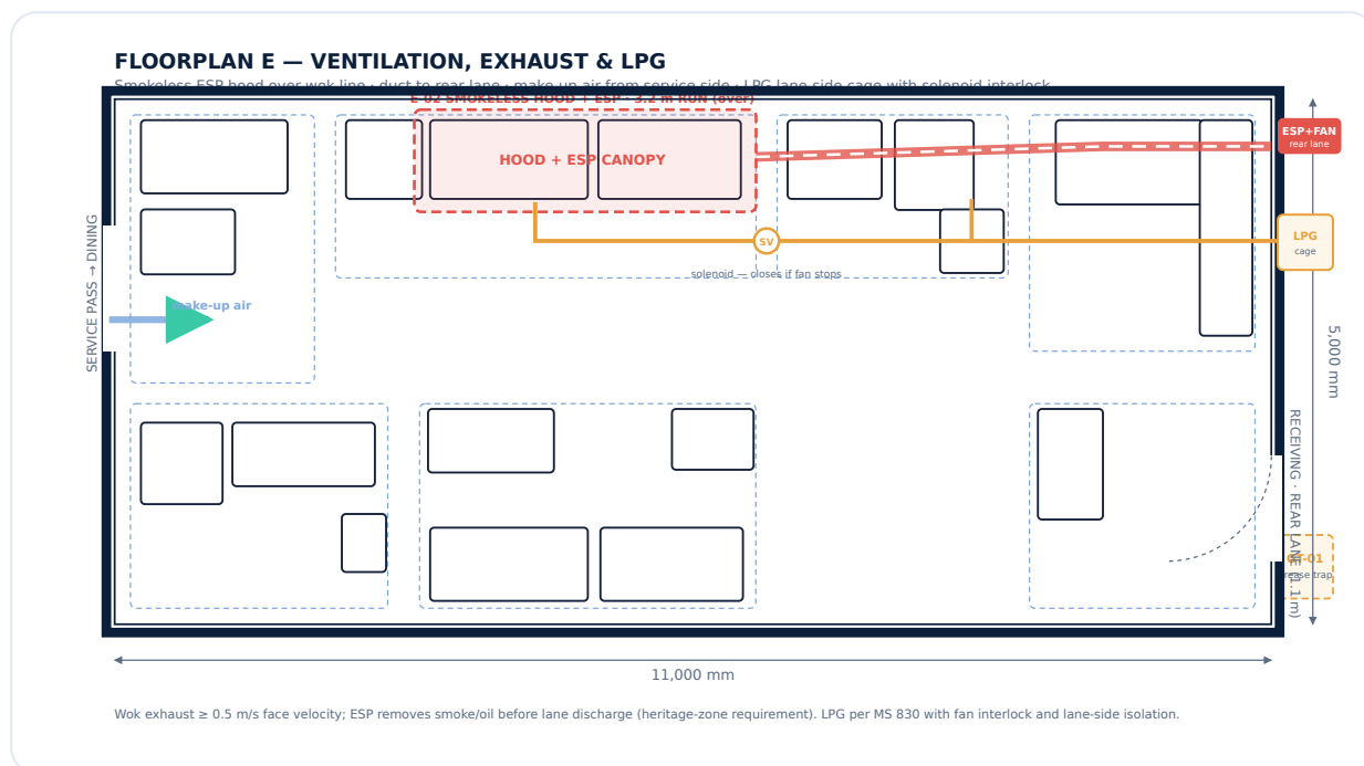
Floorplan E — exhaust route, make-up air and interlocked LPG reticulation.
