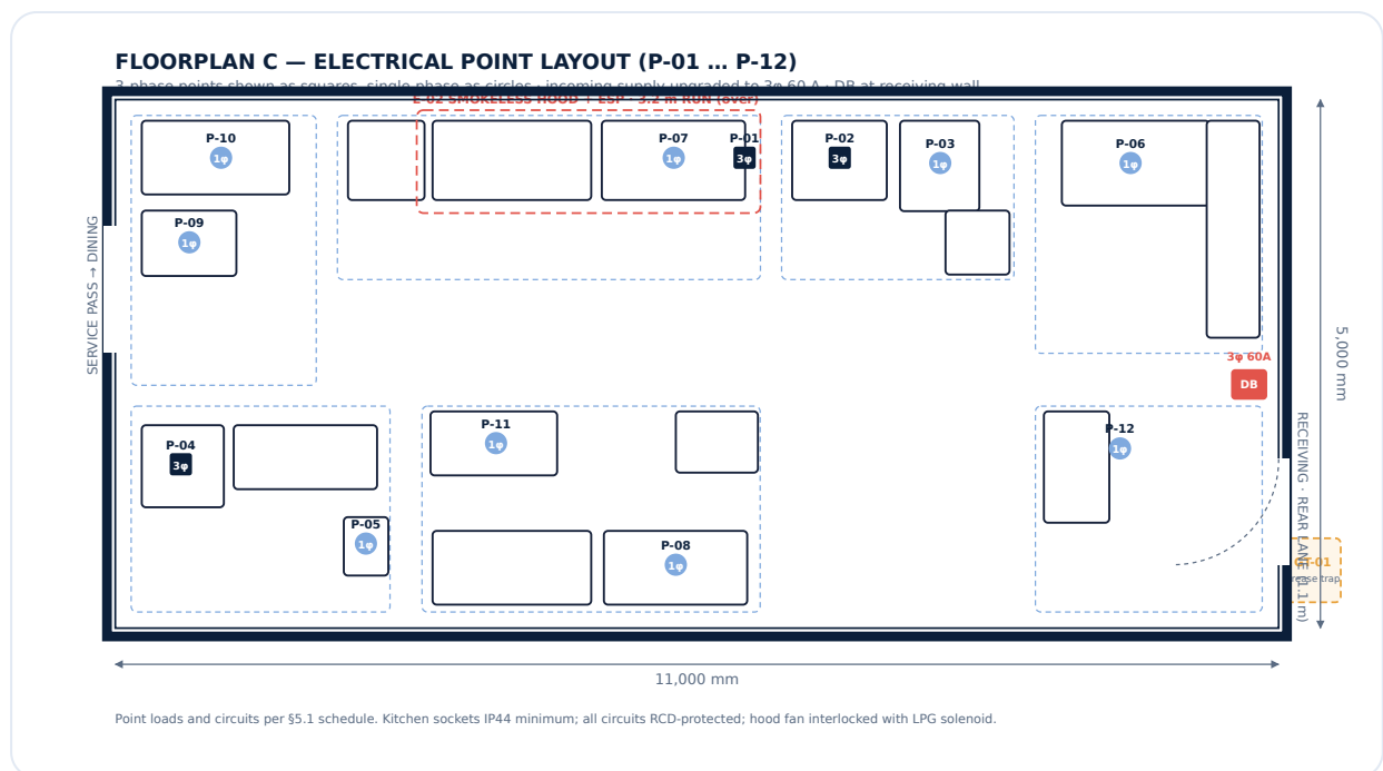
Floorplan C — electrical points. ■ 3-phase · ● single-phase · DB = distribution board.
