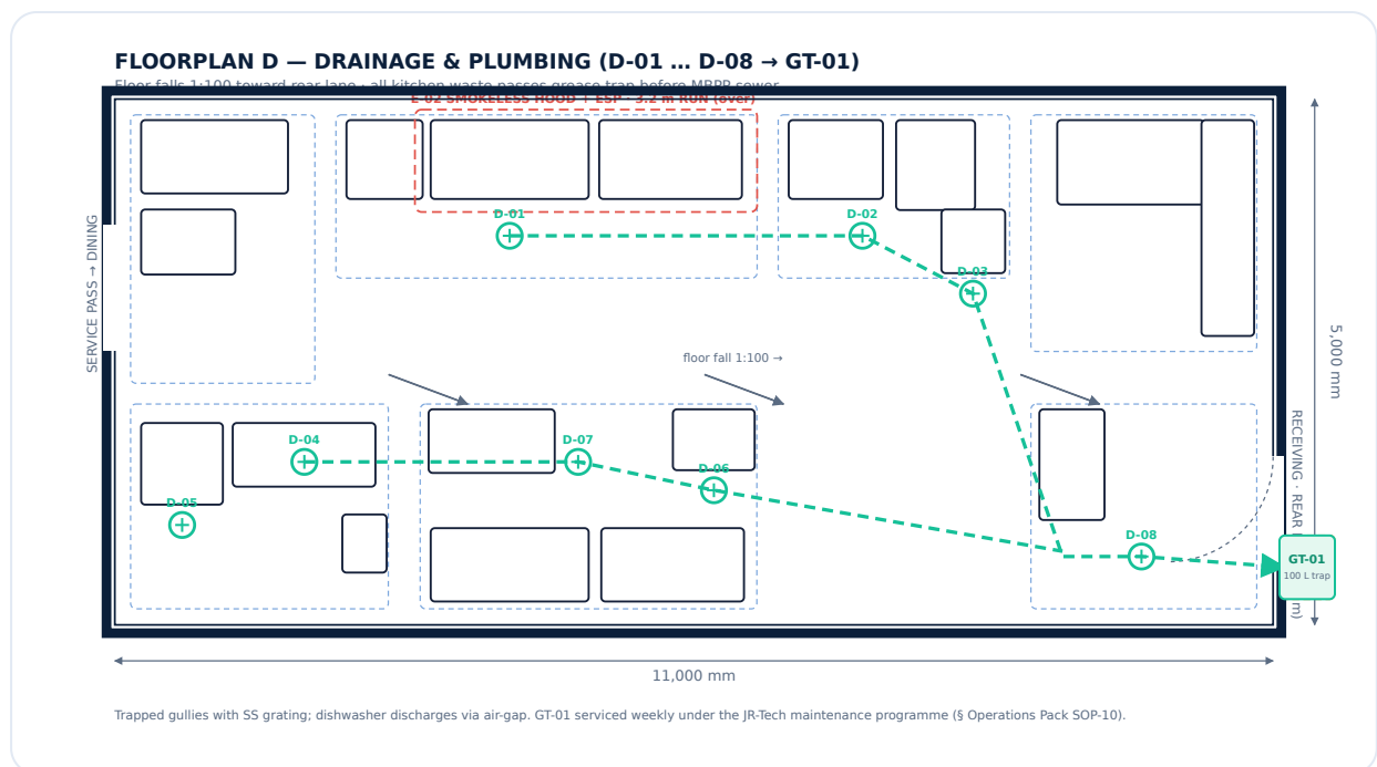
Floorplan D — drainage runs, floor falls and the lane-side grease trap.
