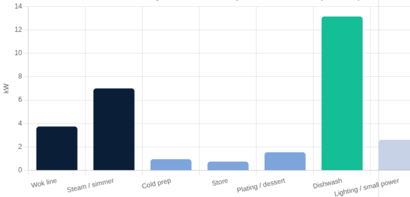
Electrical connected load by zone — total 29.75 kW (woks, steamer and stock pot on LPG)
