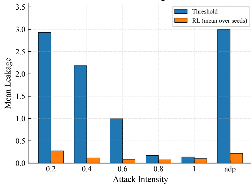
DOS - Leakage
