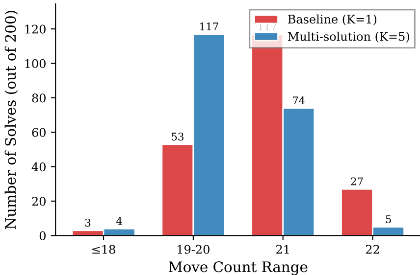
Solution Length Distribution: K=1 vs K=5
