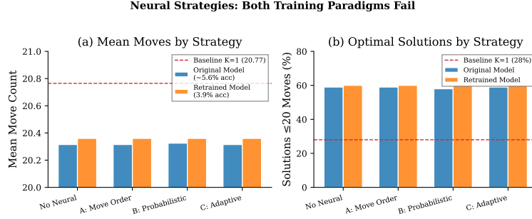
Fig. 8: Neural strategy comparison. Neither scalar-feature model nor solver-feedback retrained model improves over the non-neural baseline. Error bars: 95% bootstrap CIs.
