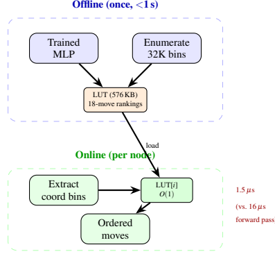
Fig. 10: LUT pipeline. Offline: enumerate all 32K coordinate bins, run the MLP once for each, store 18-move rankings (576 KB). Online: each node does an O(1) array lookup instead of a neural forward pass.
