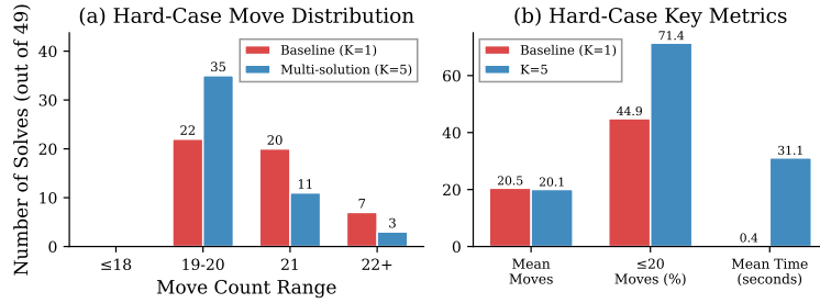
Fig. 12: Hard cases ( K=1 vs. K=5 ): move distribution and key metrics.
