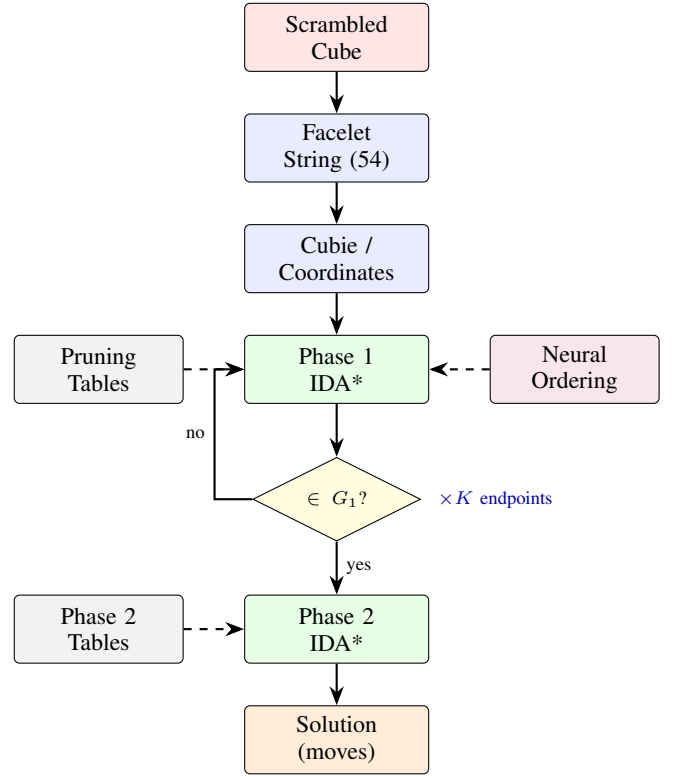
Fig. 1: Solver pipeline. The scrambled cube is converted to coordinates, then Phase 1 searches for states in subgroup G_1 (optionally guided by neural ordering). Phase 2 completes the solve. With K > 1 , multiple Phase 1 endpoints are tried and the shortest overall solution is kept.
