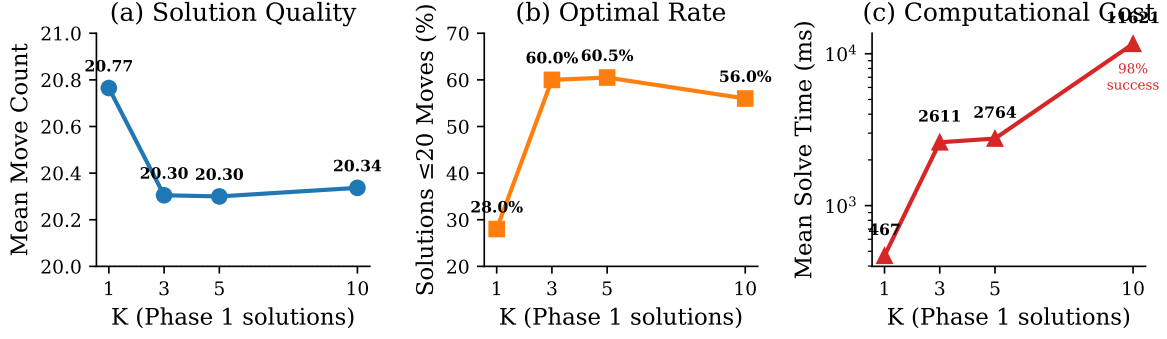
Fig. 4: Effect of K on solution quality, optimality rate ( \leq 20 moves), and solve time. Quality improves sharply from K=1 to K=3 , then plateaus.
