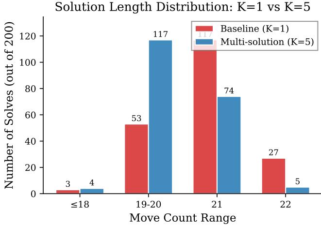
Fig. 5: Solution length distribution: K=1 vs. K=5 . Multi-solution search shifts mass from 21–22 moves toward \leq 20 moves.
