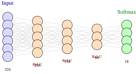
Fig. 3: Move predictor MLP. The one-hot encoding (324 dims) or coordinate features (161 dims) pass through three hidden layers. The 18-way softmax output gives a distribution over moves for ordering.
