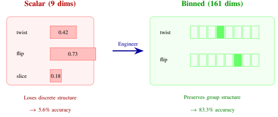
Fig. 8: Feature representation comparison. Scalar coordinates normalise to [0, 1] , destroying discrete structure (5.6% accuracy). Binned one-hot encoding preserves structural regions (83.3% accuracy)—a 15\times improvement with the same MLP.
