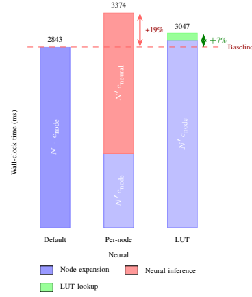
Fig. 10: Inference overhead barrier. Default (2843 ms): node expansion only. Per-node neural (3374 ms): 2.4\times fewer nodes but +19% overhead from inference cost. LUT (3047 ms): same idea, but O(1) lookup replaces the forward pass, cutting overhead to +7%.
