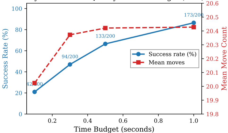
Anytime Search: Quality vs Time Budget (K=5)
