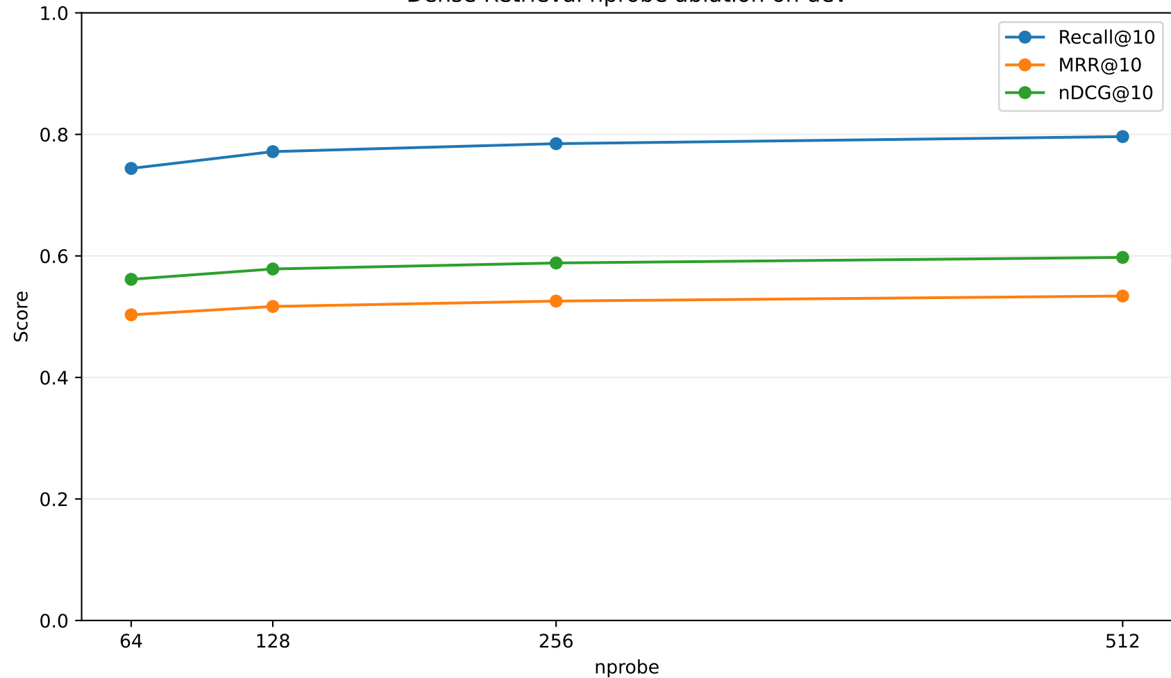
Dense Retrieval nprobe ablation on dev
