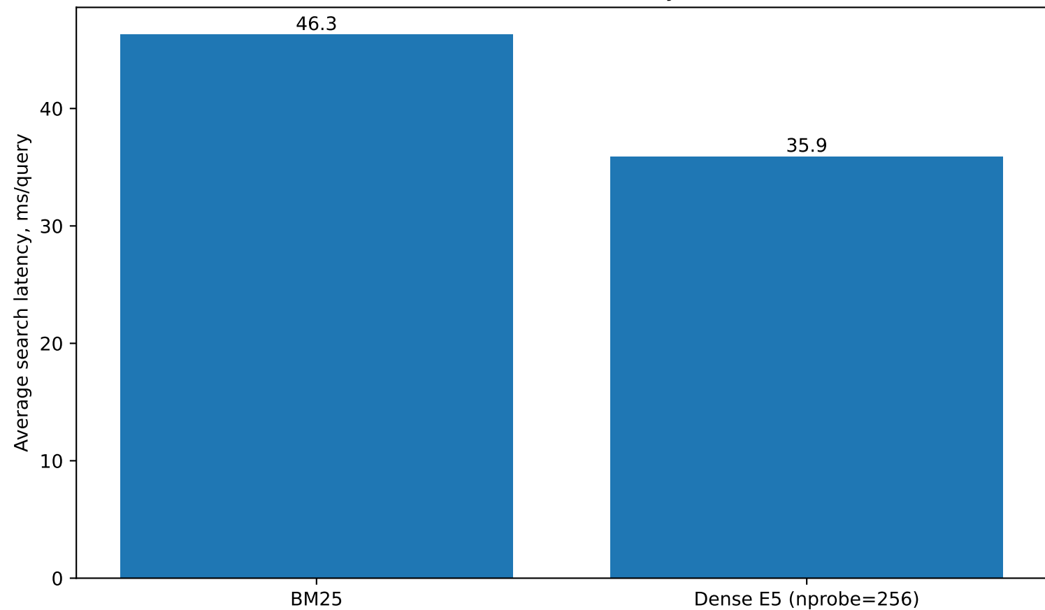
Test retrieval latency
