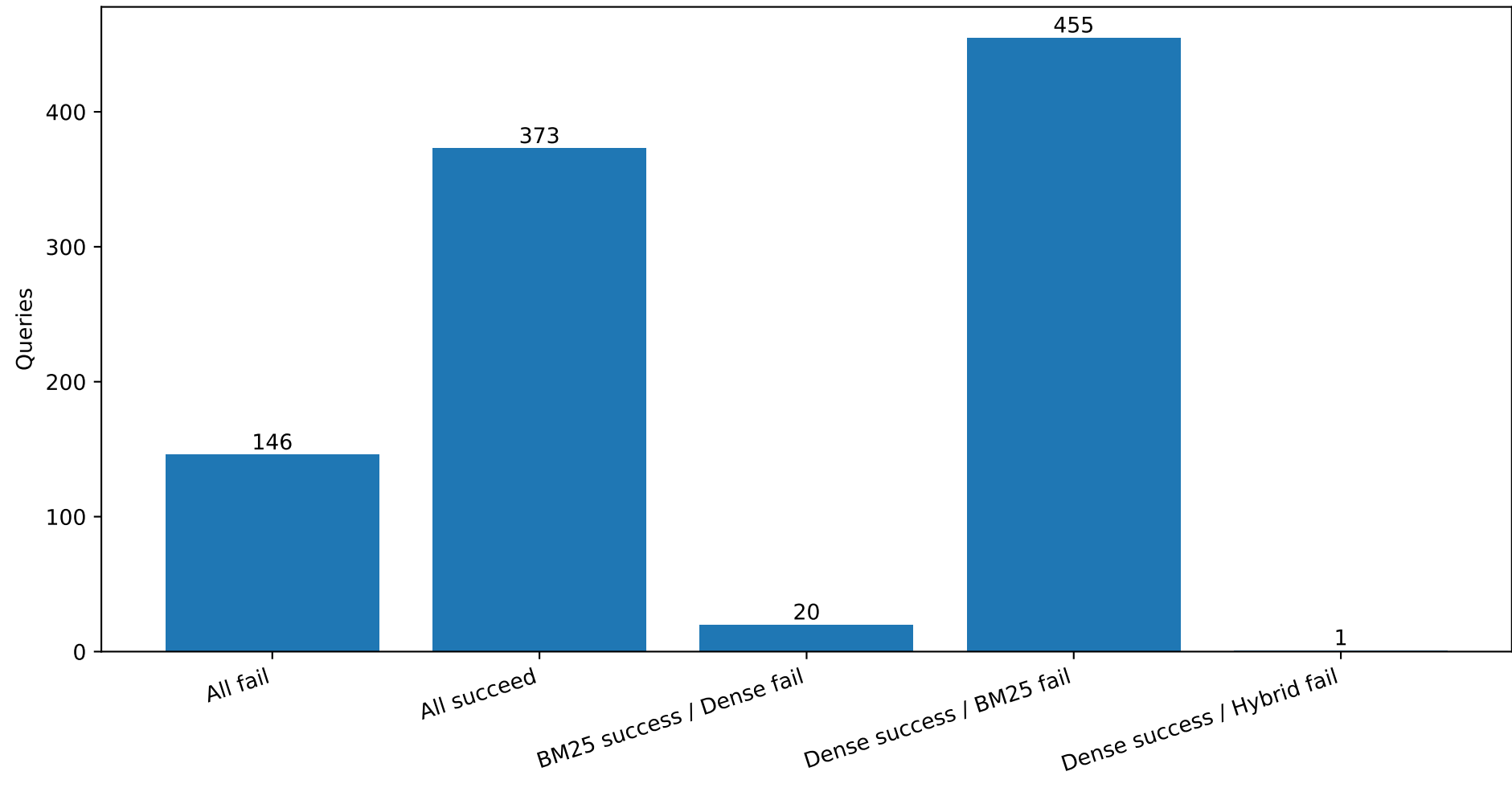
Test error-analysis categories
