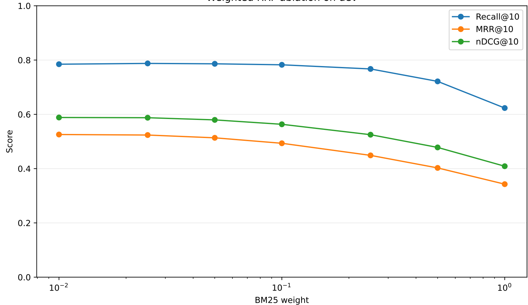
Weighted RRF ablation on dev
