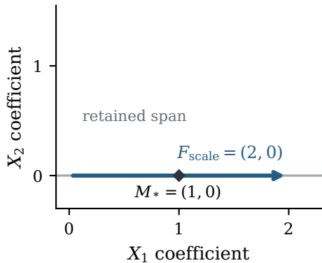
(a) Decoder magnitude error
