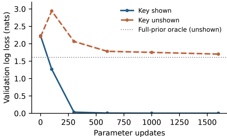
Query-prediction training
