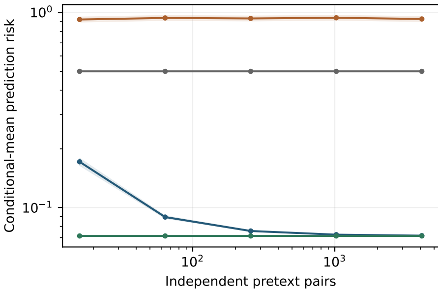
10 task labels
