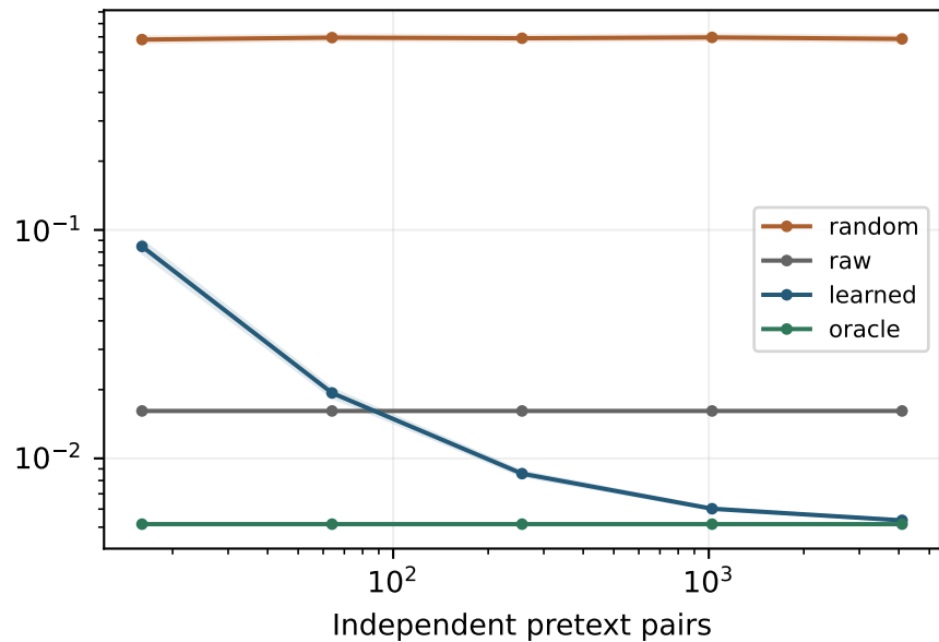
100 task labels
