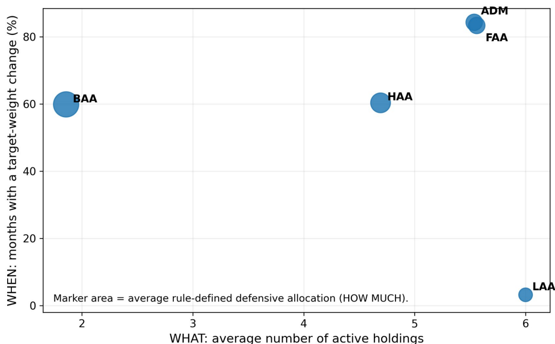
Figure 2. Decision fingerprints: What, When, and How Much. The dimensions are descriptive rather than a single optimized score. Their purpose is to reveal which kinds of disagreement each sleeve adds.
