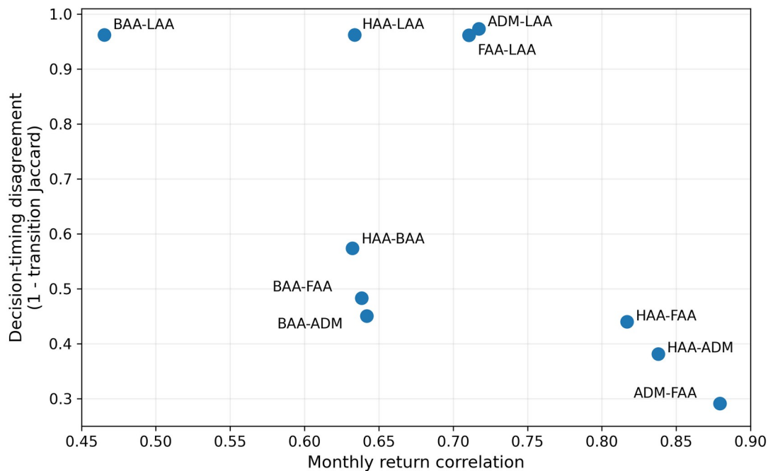
Figure 1. Similar returns do not imply similar decisions. The horizontal axis shows monthly return correlation. The vertical axis shows disagreement in portfolio-transition timing, measured as one minus the share of transition months common to both strategies (Jaccard overlap). A value near one means the pair rarely changes its target weights in the same month. Return correlation remains useful, but it does not fully describe how rules behave.
