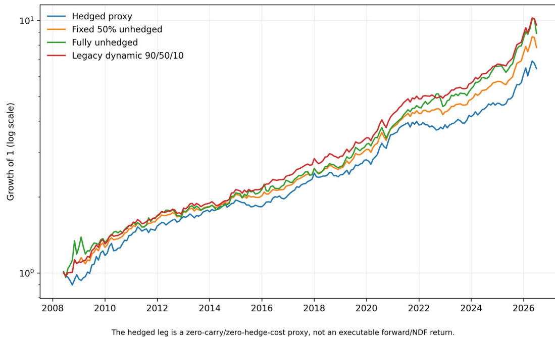
Appendix FX Figure 1. KRW/USD currency-exposure variants. The figure compares growth of one under the gross underlying ADAA path with four currency-exposure choices. The “hedged” path is a zero-carry and zero-hedge-cost proxy. It is not an executable forward or NDF return.
