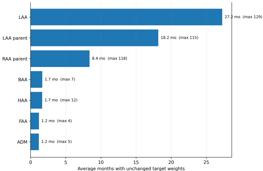
Figure 3. Different rules operate on different decision clocks. The current HAA and BAA targets remain unchanged for roughly 1.7 months on average; ADM and FAA for about 1.2 months. Current ADAA-LAA remains unchanged for about 27 months on average. The source LAA and the out-of-portfolio RAA comparator are also materially more persistent than the faster dynamic sleeves.
