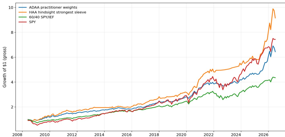
Figure 6. Cumulative wealth makes the trade-off visible. Growth of $1 is shown for gross ADAA using the later practitioner weights, the hindsight-strongest HAA sleeve, the SPY/IEF 60/40 benchmark, and SPY over the common June 2008-July 2026 sample. The chart is descriptive: it shows the path behind the summary statistics, not a claim that ADAA maximizes terminal wealth.
