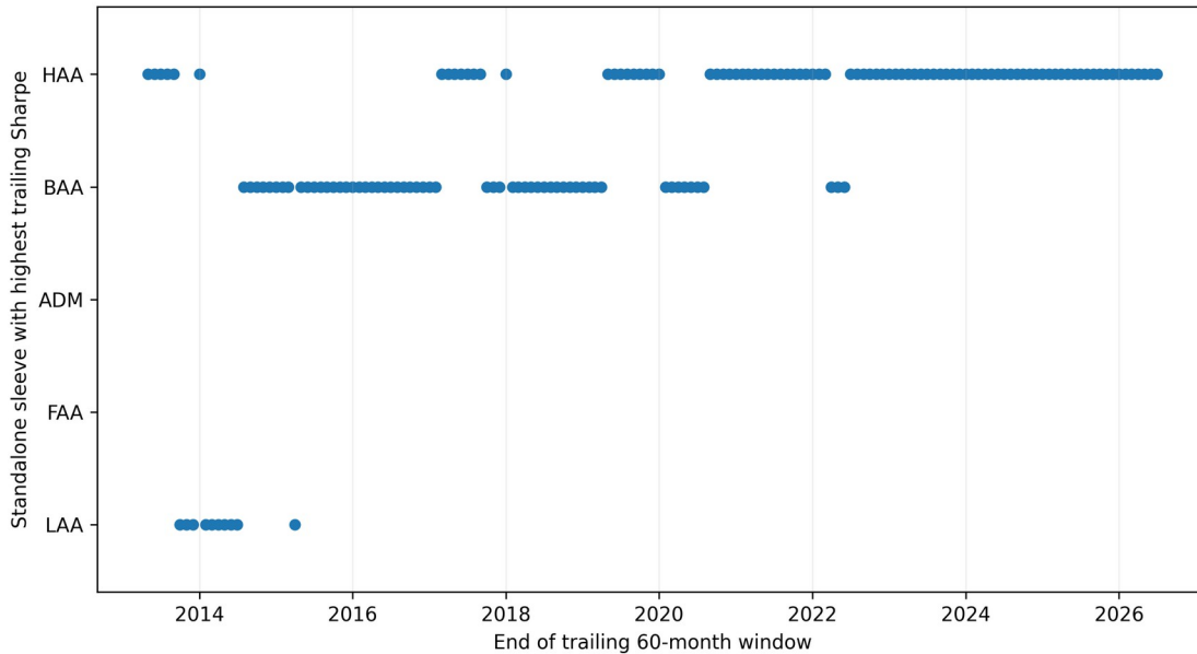
Figure 4. The hindsight winner changes as the window moves. Each point identifies the standalone sleeve with the highest trailing 60-month BIL-excess Sharpe. The chart is not a timing strategy and does not allow ex-post switching. It illustrates model uncertainty: the rule that looks best depends on where the evaluation window ends. ADA using the later practitioner weights is above the median constituent in 98.7% of 60-month Sharpe windows, top-two in 69.2%, and bottom-two in 0%.
