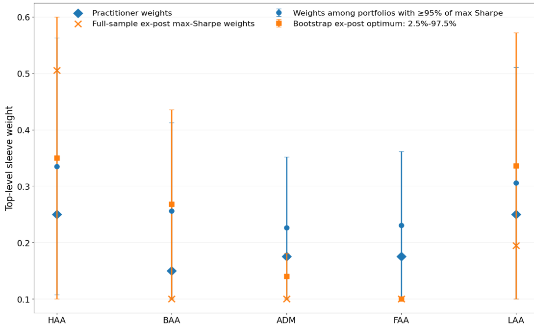
Figure 5. The near-optimal weight region is broad, while the estimated optimum moves. The near-optimal ranges are descriptive properties of the fixed full sample, not confidence intervals. The bootstrap ranges show how much the ex-post optimum moves when the historical path is resampled in 12-month blocks. About 40.3% of the 100,000 weight vectors satisfying the minimum-weight constraint retain at least 95% of the full-sample maximum Sharpe.
