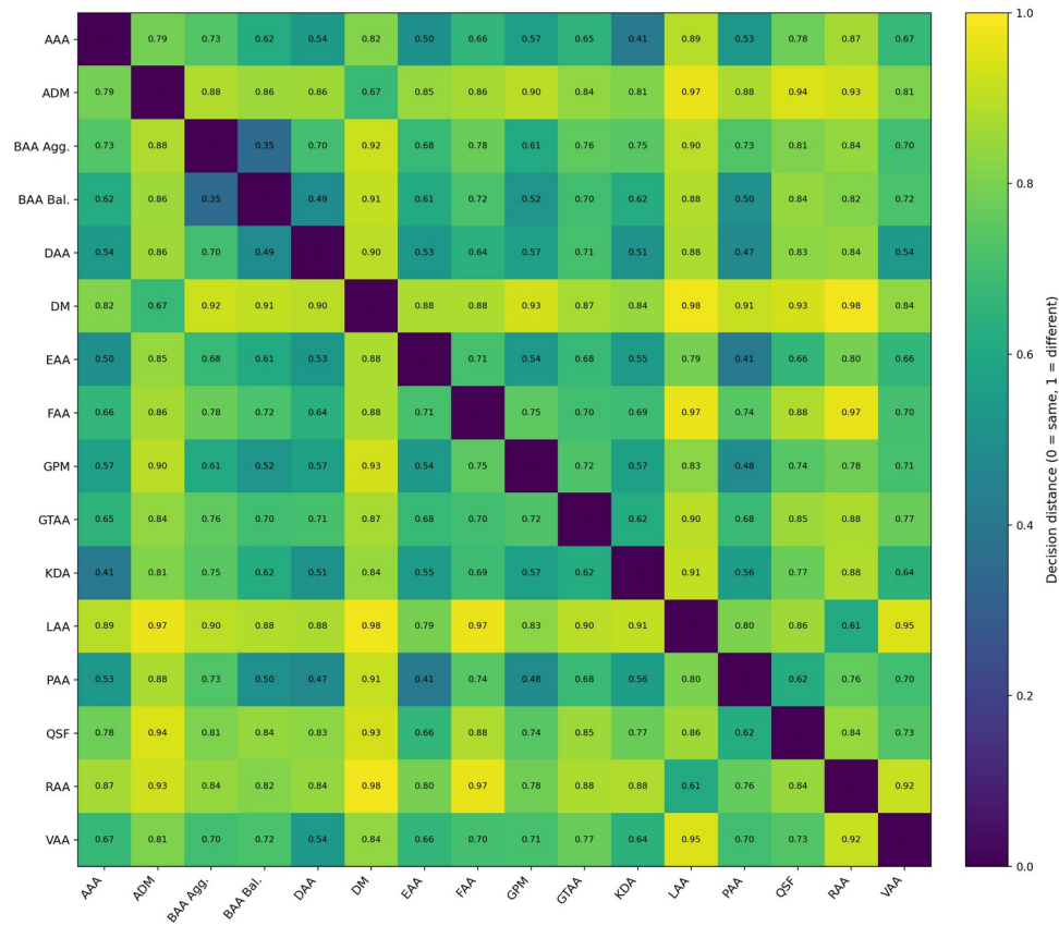
Appendix Figure Z1. The 2023 Strategy Zoo in Decision Space. Lower values mean more similar portfolio decisions; higher values mean greater disagreement in target allocations, holdings, and transition dates. No strategy-performance statistic enters the matrix.
