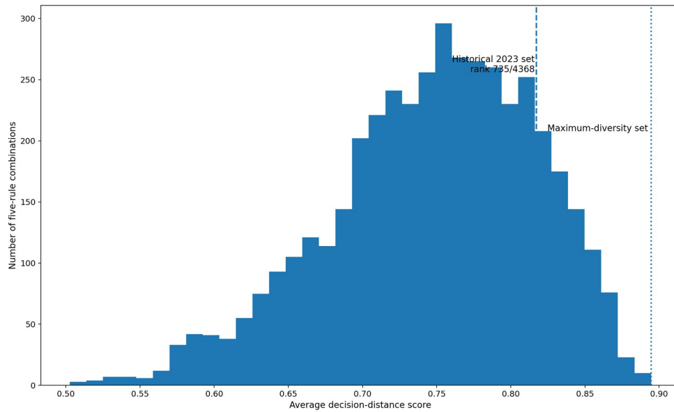
Appendix Figure Z2. Historical ADAA was highly decision-diverse, but not maximally diverse. Bars count the 4,368 feasible five-rule combinations by Decision-Space score. Higher scores mean greater decision disagreement, not better returns; the figure is not a performance test.
