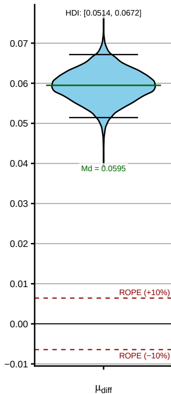
RMSE
