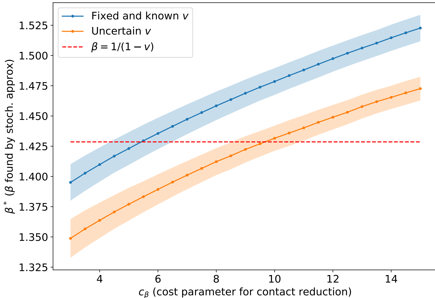
Problem 2. Solution \beta^* as a function of cost parameter v = 0.3, N = 1000, T = 10
