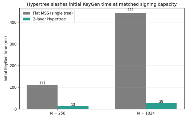
Figure 10: Initial KeyGen time: flat MSS vs 2-layer hypertree at matched signing capacities. The hypertree is 8.2\times faster at N=256 and 15.6\times faster at N=1024 , confirming the predicted O(\sqrt{N}) behavior.
