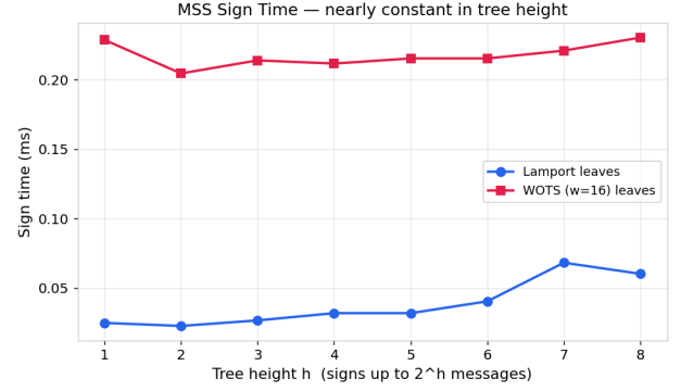
(b) MSS Sign time vs. height.
