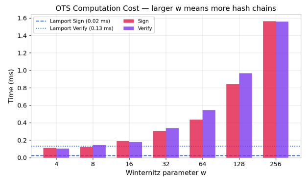
(b) Sign and verify times vs. w .
