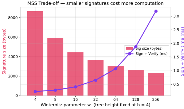
Figure 4: MSS size-vs-speed trade-off at h=4 . The knee near w = 16 marks the practical sweet spot adopted by XMSS and SPHINCS+.
