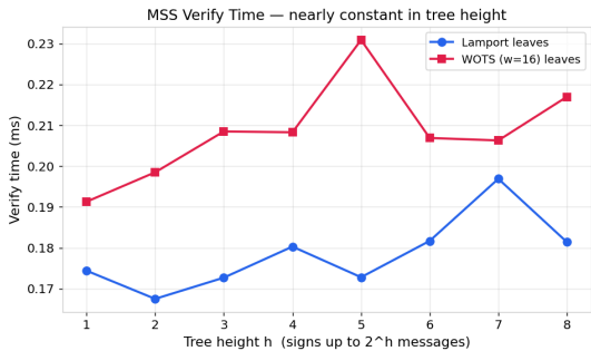
(c) MSS Verify time vs. height.
