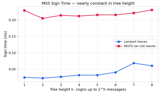
(b) MSS Sign time vs. height.
