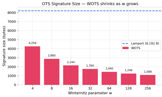
(a) Signature size vs. w .
