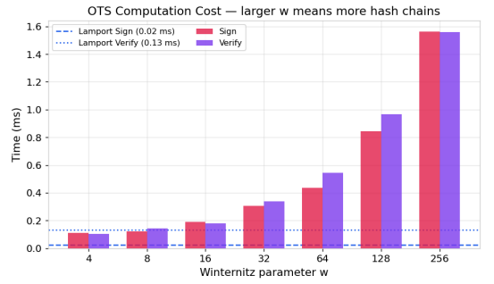
(b) Sign and verify times vs. w .
