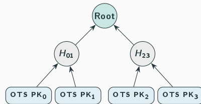
Lamport or WOTS public keys as leaves
