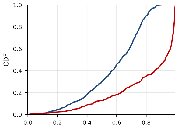
(c) Pearson-r
