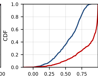
(f) Pearson-r
