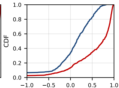
(c) KGE
