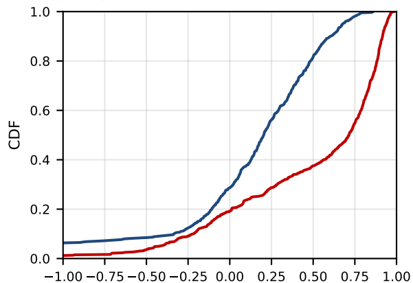
(b) KGE
