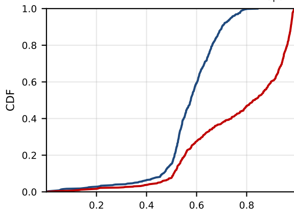
(a) NNSE
