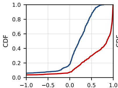
(a) NSE
