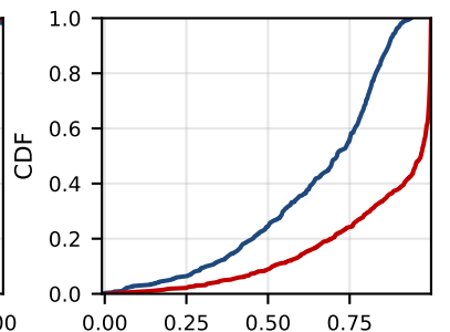
(f) Pearson-r
