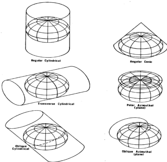
Figure 1.4 The geometric constructions of projections using developable surfaces 19/39
