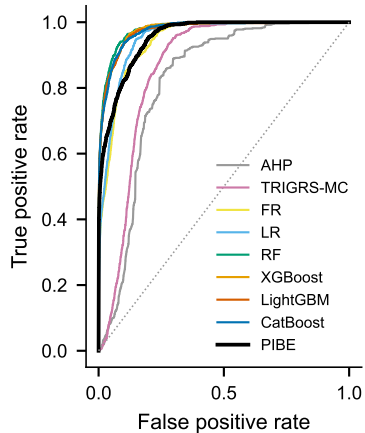
(a) ROC, spatial CV
