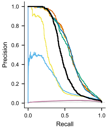
(b) Precision-recall
