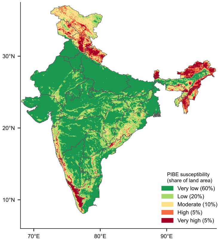
(a) National landslide susceptibility (0.05°)
