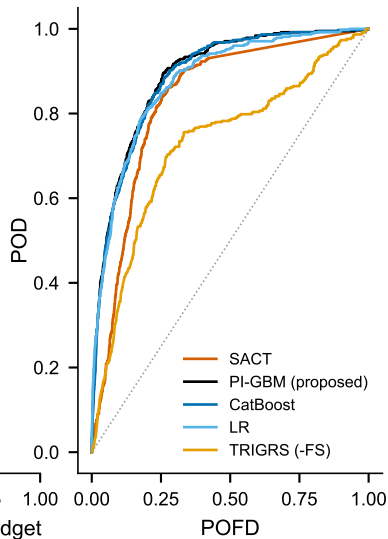
(c) ROC, test 2013-2025
