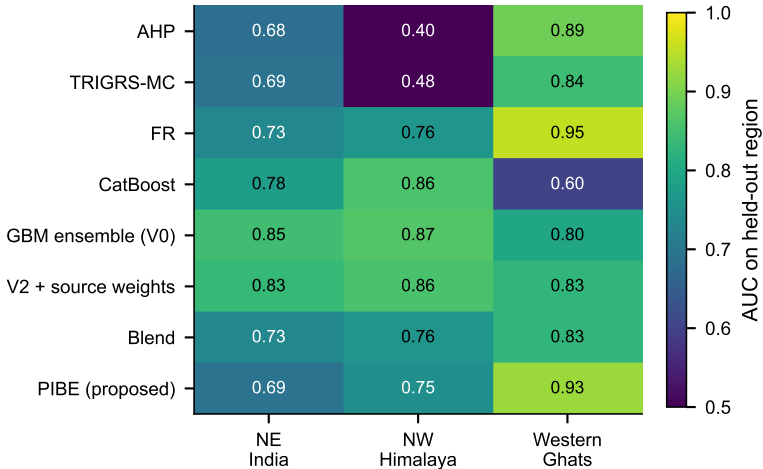
Leave-one-region-out transfer
