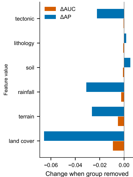
(b) Factor-group ablation
