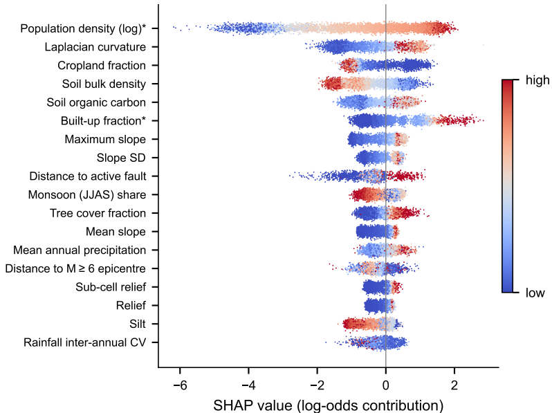
(a) SHAP, bias-aware member of PIBE (*fixed when mapping)
