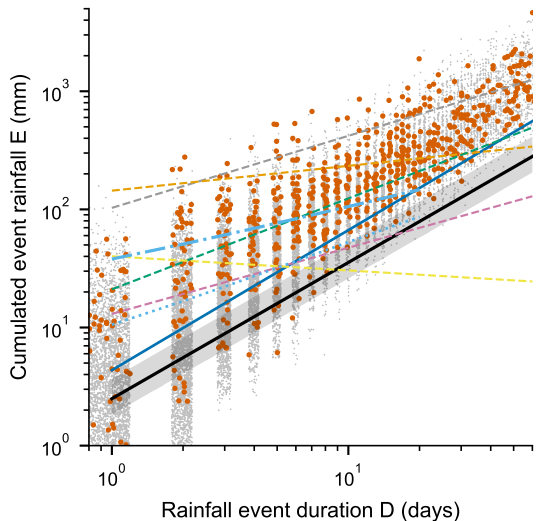
(a) Empirical and physical thresholds
