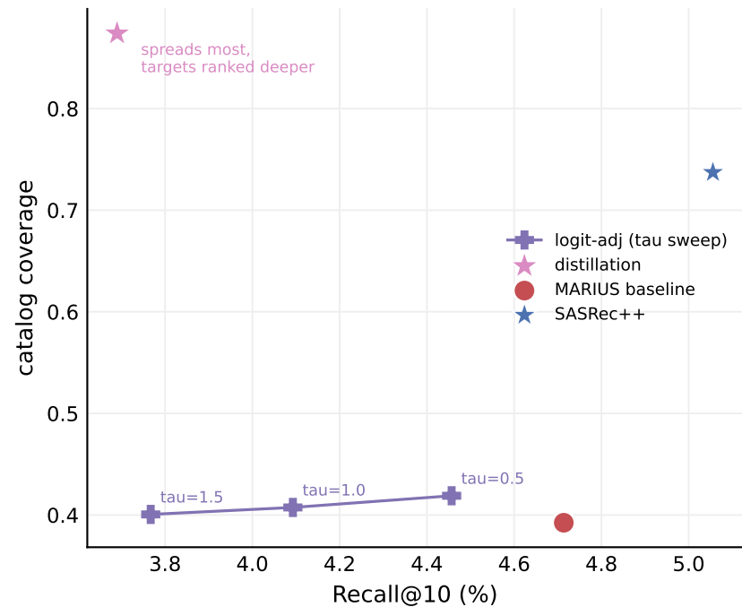
C. Sports (18k): logit-adj + distillation
