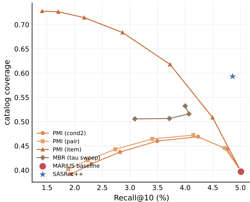
A. Arts (90k): post-hoc PMI / MBR re-rank
