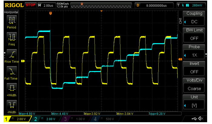
Fig. 8: Modulation pattern acquired using Sagnac Development Kit presents an 18b-DAC operating at f=1\text{MHz} . Yellow waveform is the biasing sequence, symmetrical around zero. Even with a low resolution DAC determining errors at the lsb level would not be possible visually. The cyan waveform in the nulling ramp with Serrodyne reset at 2\pi .
