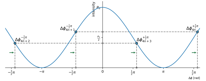
(c) Phase shift induced by rotation in one direction - bias points shifted right. Points \{4n, 4n + 1\} result in higher intensity than points \{4n + 2, 4n + 3\} .
