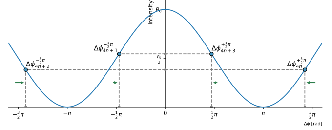
(b) Scale factor too low - bias points shifted towards zero, resulting in opposite imbalance.
