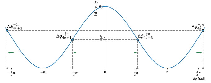
(a) Scale factor too high - bias points are shifted away from zero, resulting in intensity imbalance.
