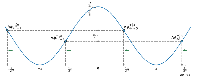
(d) Phase shift induced by rotation in opposite direction - bias points shifted left. Points \{4n, 4n + 1\} result in lower intensity than points \{4n + 2, 4n + 3\} .
