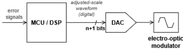
Fig. 6: All-digital modulator consists of minimal number of electronic components. In some applications this can simply be a DAC alone.
