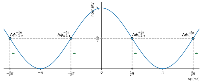
Fig. 3: Circuit biased in four points of highest sensitivity.
