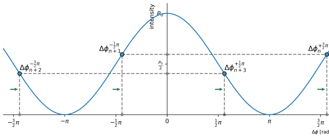
(c) Phase shift induced by rotation in one direction - bias points shifted right. Points \{4n, 4n+1\} result in higher intensity than points \{4n+2, 4n+3\} .
