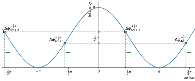
(d) Phase shift induced by rotation in opposite direction - bias points shifted left. Points \{4n, 4n+1\} result in lower intensity than points \{4n+2, 4n+3\} .
